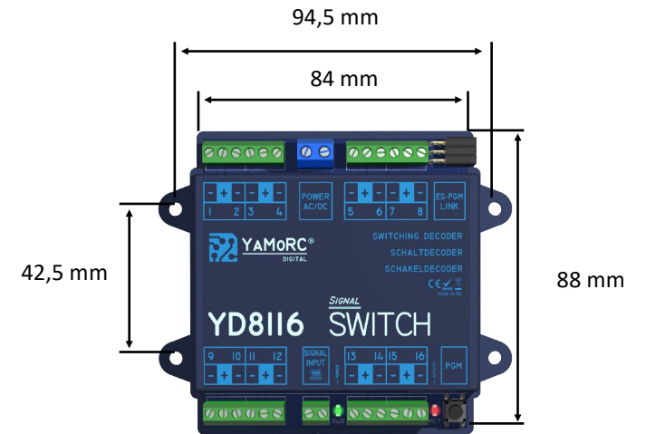
Dimensional Drawing
